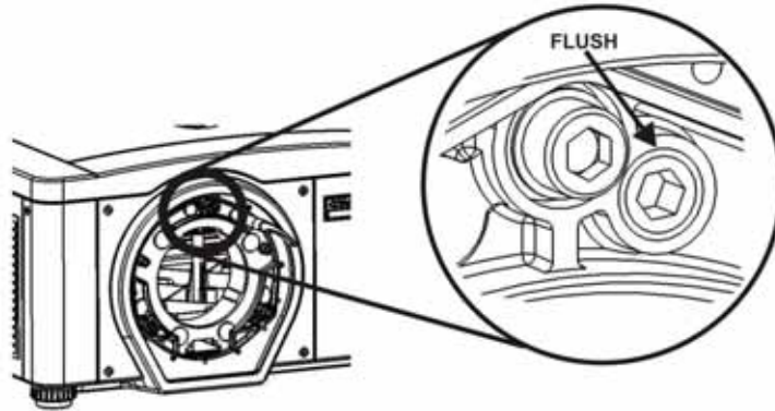
FIGURE 2-5 POSITION SETSCREW FLUSH
