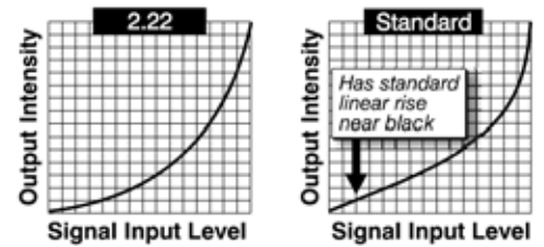
FIGURE 3-9 GAMMA CURVE
