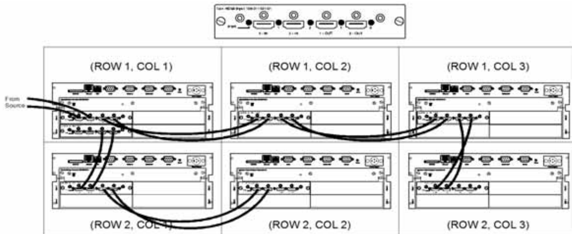
FIGURE 2-10 2X3 LOOP-THROUGH WIRING SOLUTION
