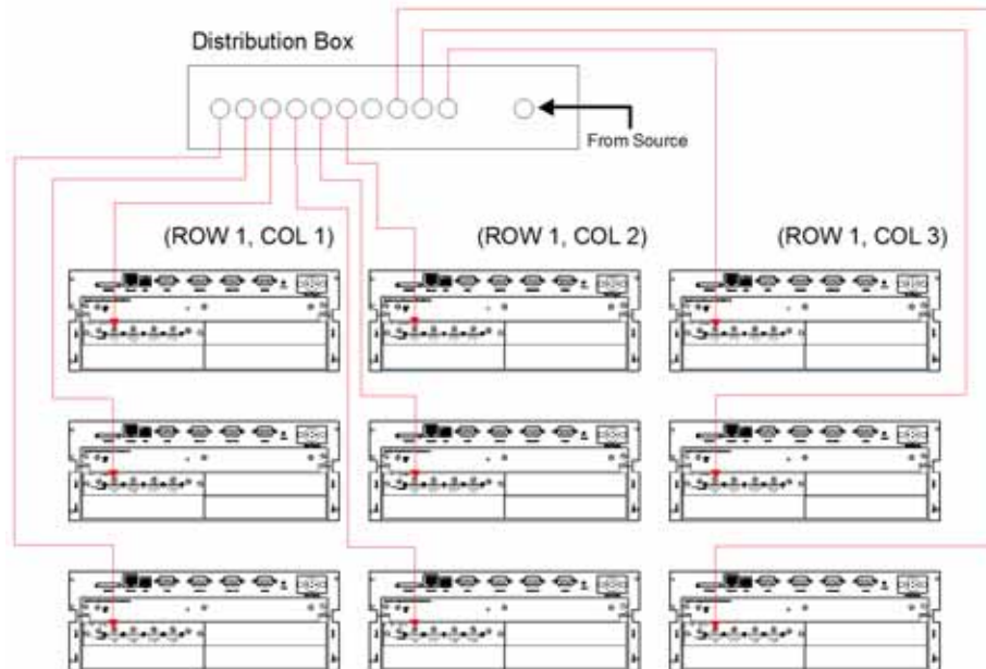
FIGURE 2-7 USE OF DISTRIBUTION BOX
