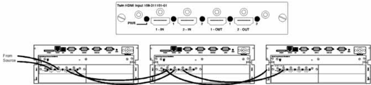
FIGURE 2-8 1X3 WIRING SOLUTION
