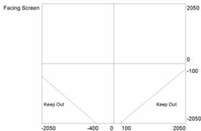
FIGURE B-1 LENS CONTROL LIMITATIONS
