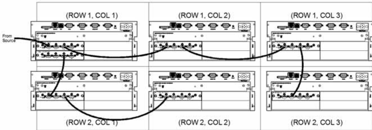
FIGURE 2-11 2X3 SINGLE WIRING LOOP-THROUGH - NO PIP IS SUPPORTED
