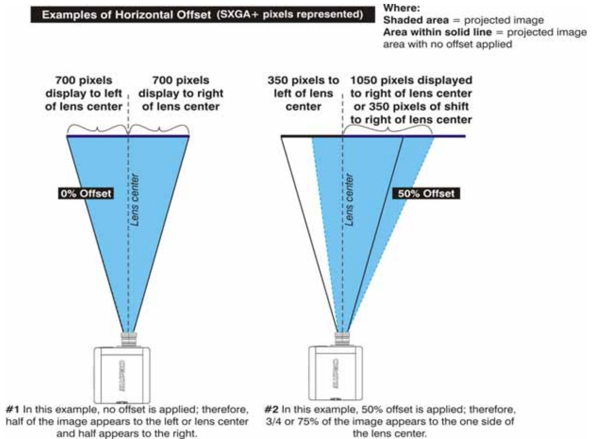
FIGURE 2-2 HORIZONTAL OFFSET EXAMPLES
