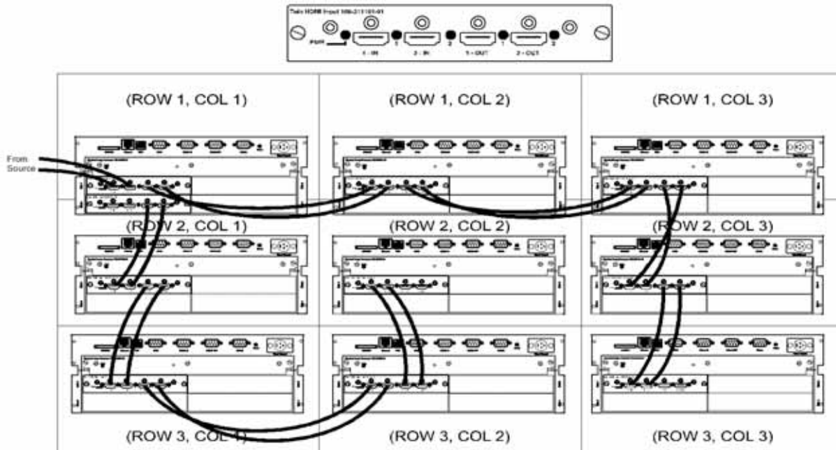
FIGURE 2-12 3X3 LOOP-THROUGH WIRING SOLUTION
