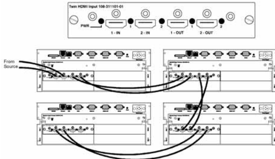
FIGURE 2-9 2X2 WIRING SOLUTION
